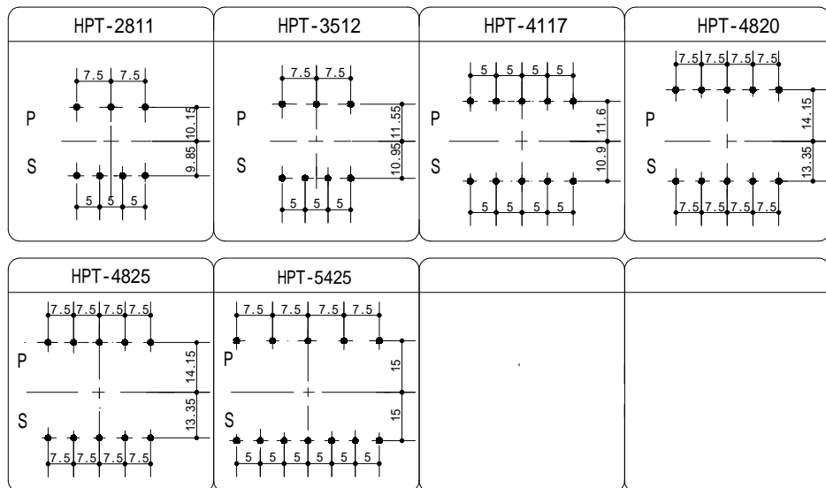
端子間隔 (Bottom View)
