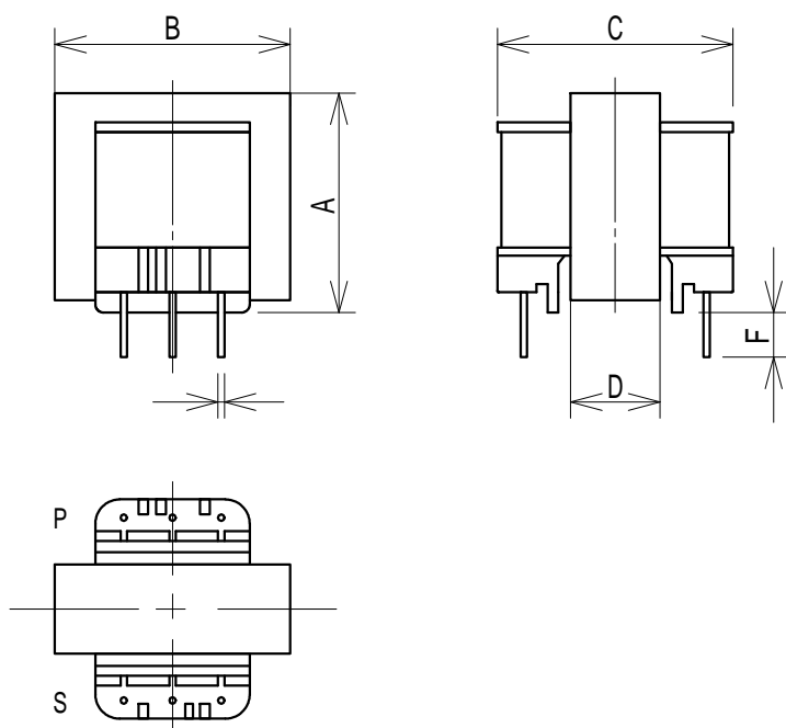
端子間隔 (Bottom View)
